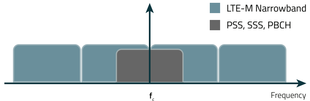
Figure 3: Arrangement of LTE-M narrowbands for a 5-MHz carrier
